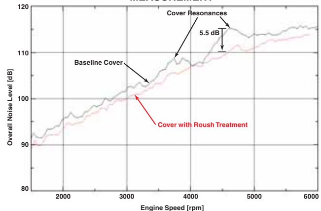
FIGURE 2: NEARFIELD SOUND PRESSURE MEASUREMENT
